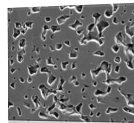
Reactive Sintering
